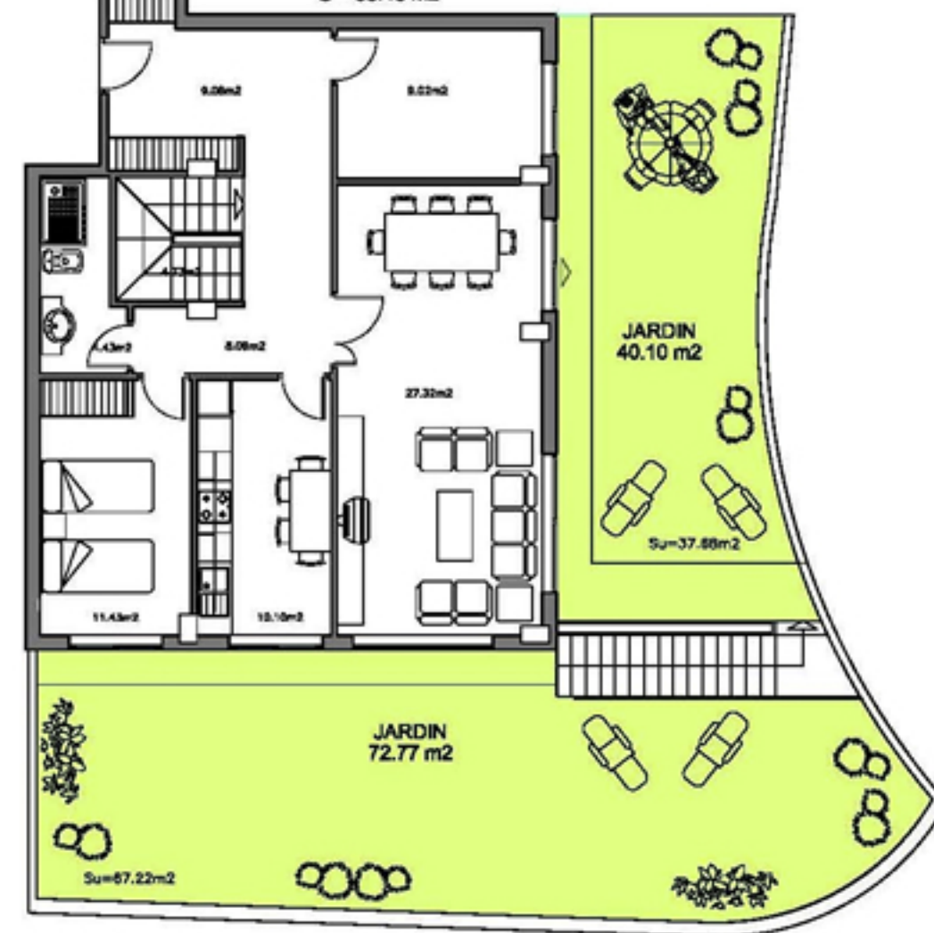
DUPLEX E Su=84.20 m 2 S = 95.43 m 2
